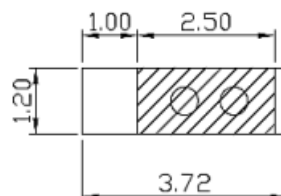
RECOMMENDED PAD FOR THE PCB (mm)
