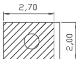
RECOMMENDED PAD FOR THE PCB (mm)
