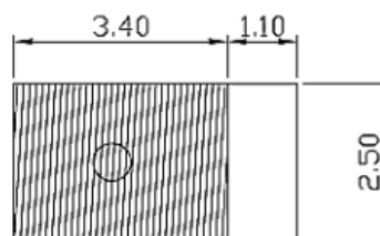
RECOMMENDED PAD FOR THE PCB (mm)
