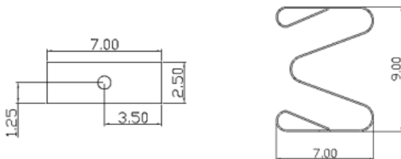
RECOMMENDED RESERVED AREA ON THE PCB (mm)
