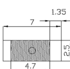
RECOMMENDED PAD FOR THE PCB (mm)
