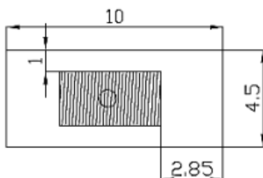
RECOMMENDED RESERVED AREA ON THE PCB (mm)
