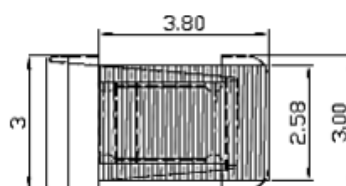
RECOMMENDED PAD FOR THE PCB (mm)
